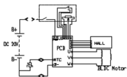
Electric circuit
